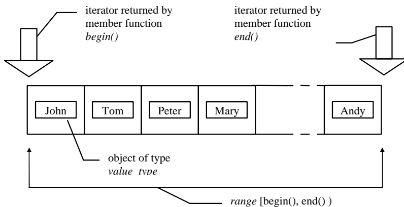
Figure 5: Range specified by iterators
