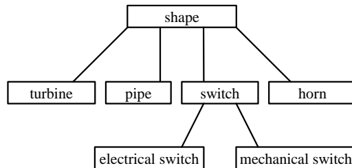
Figure 4: Example shape class hierarchy
