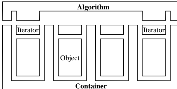
Figure 6: Orthogonal decomposition of the component space
